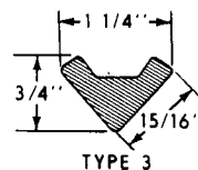
CROSS SECTION VIEW OF JACK COLUMNS
