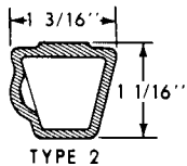
CROSS SECTION VIEW OF JACK COLUMNS
